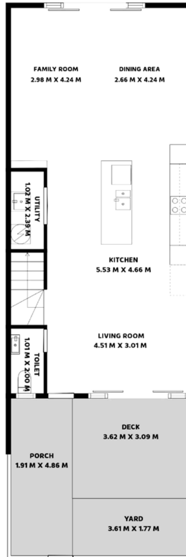
GROUND FLOOR
